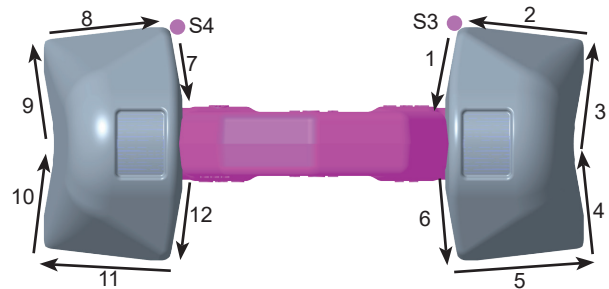
Pic. 2: Sequence of closure welding (S=Starting point)
