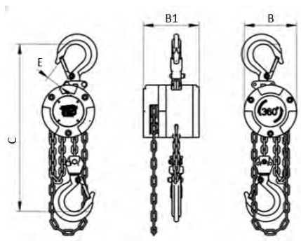
PAC Aluminium-Flaschenzug, 250 kg (Art. PAC.250)
